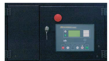
Deep Sea 7210 Control Panel
